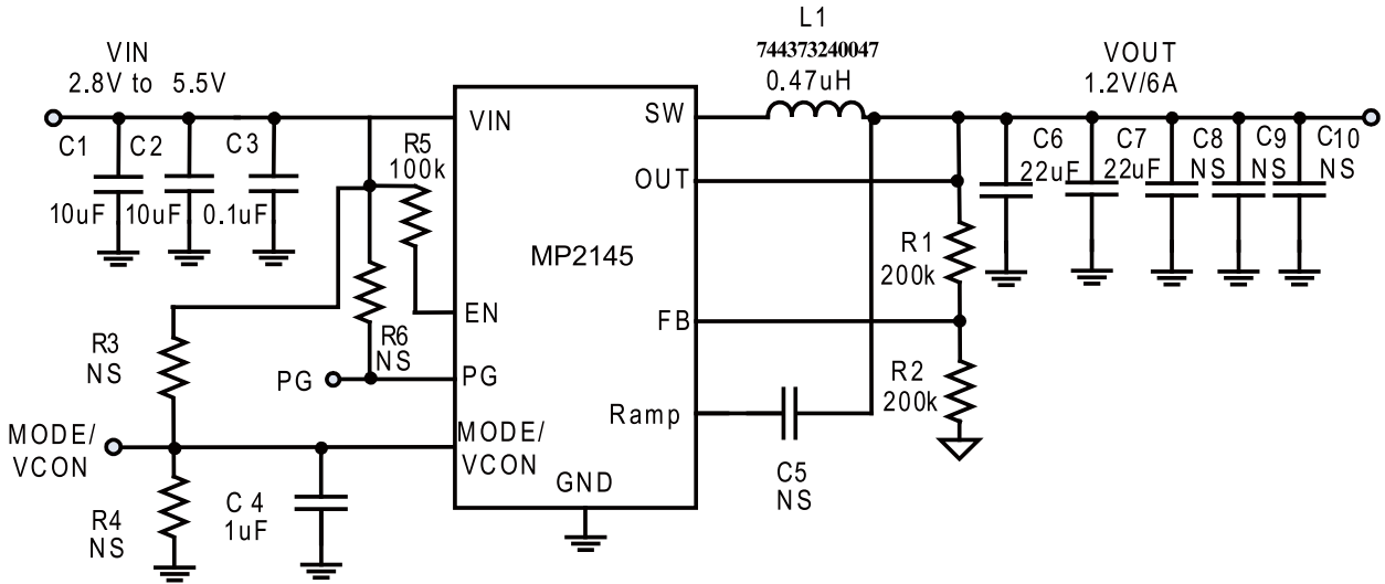
Figure 8: Typical Application Circuit for V_{IN}=5V , I_{OUT}=6A
