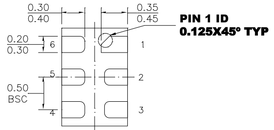
BOTTOM VIEW
