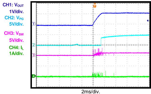
PG On I_{OUT} = 0A , PFM
