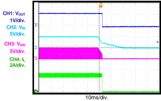
V_{IN} Shutdown I_{OUT} = 3A , PWM
