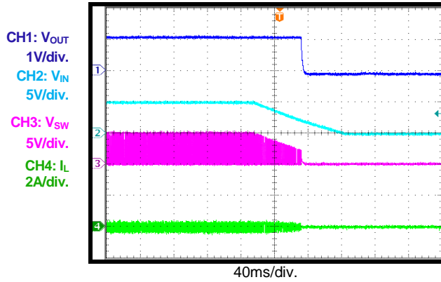
V_{IN} Shutdown I_{OUT} = 0A , PWM
