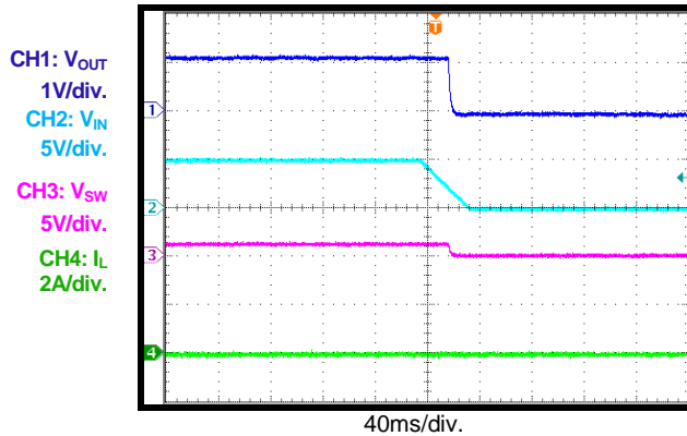
V_{IN} Shutdown I_{OUT} = 0A , PFM
