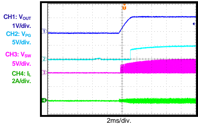
PG On I_{OUT} = 0A , PWM
