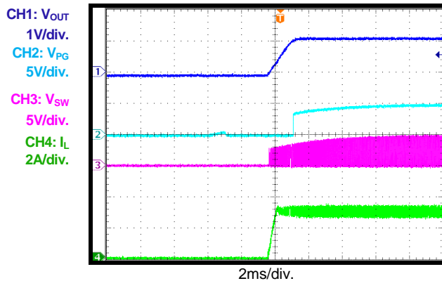
PG On I_{OUT} = 3A , PWM
