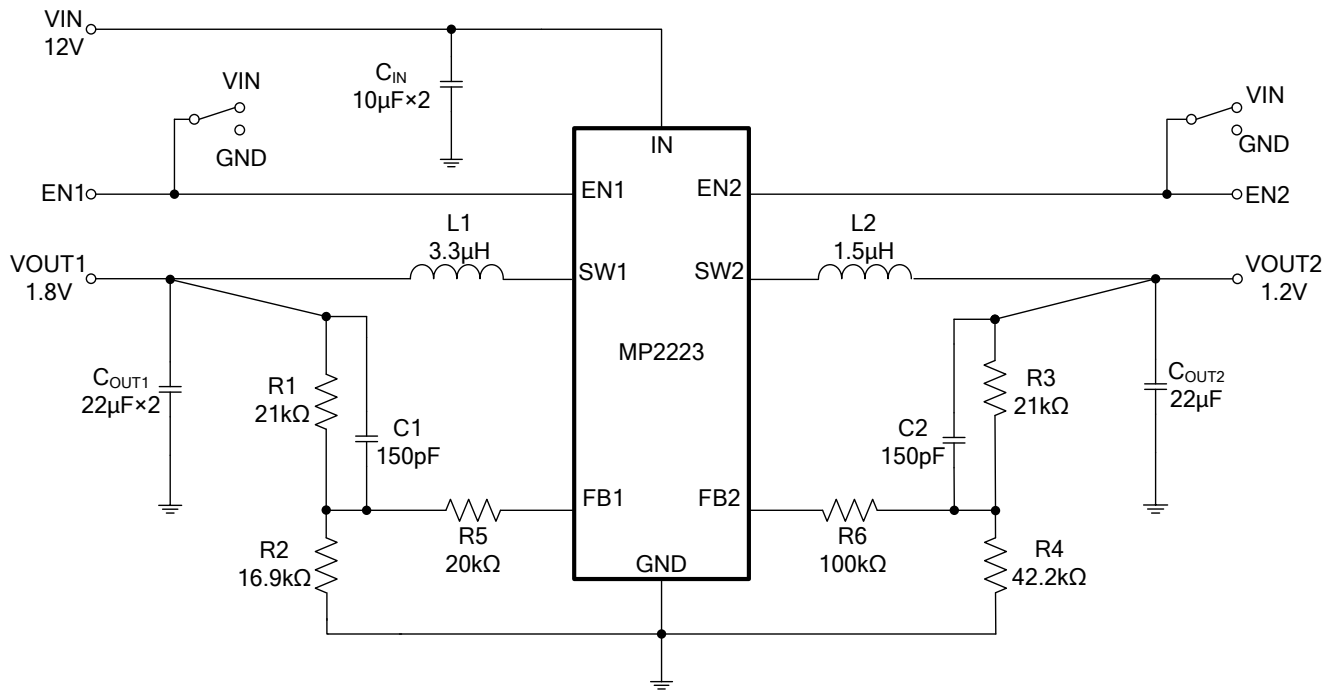
Figure 7: 12V V_{IN} , 1.8V/3A, 1.2V/2A
