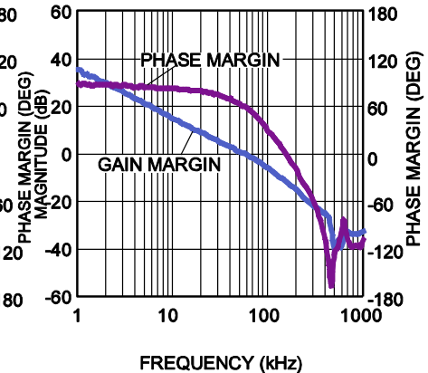
Bode Plot
