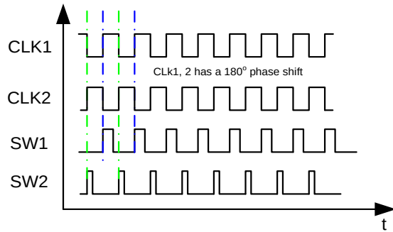
Figure 4: Clock/Switching Timing
