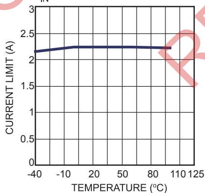
Current Limit vs. Temperature V_{IN}=19V
