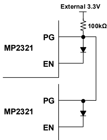
Figure 12: PG Pull up to external power supply with enable control signal --- PG parallel Output
