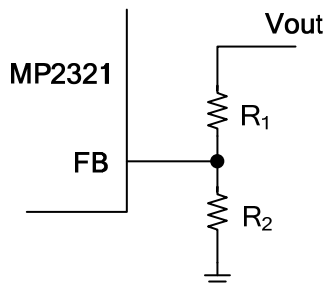
Figure 8: Feedback Network
