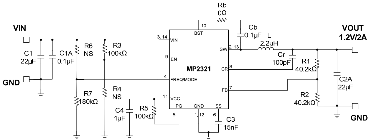
Figure 16: V_{IN} = 12V , V_{OUT} = 1.2V , I_{OUT} = 2A , F_s = 500kHz
