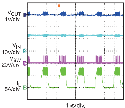
Short-Circuit Steady
