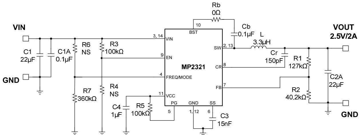
Figure 19: V_{IN} = 12V , V_{OUT} = 2.5V , I_{OUT} = 2A , F_s = 500kHz
