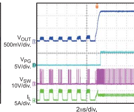
Short-Circuit Recovery
