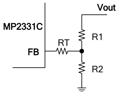
Figure 4: Feedback Network
