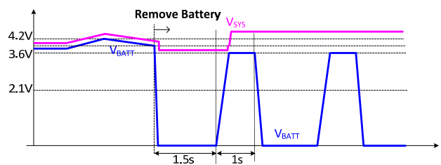
Figure 5: Battery Float Detection Examples
