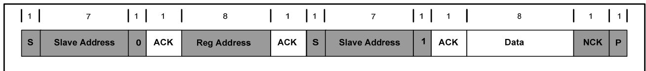
Figure 21: Single Read
