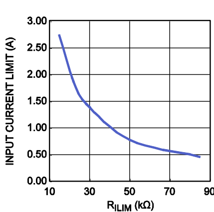
Programmable Input Current Limit, Charge Mode
