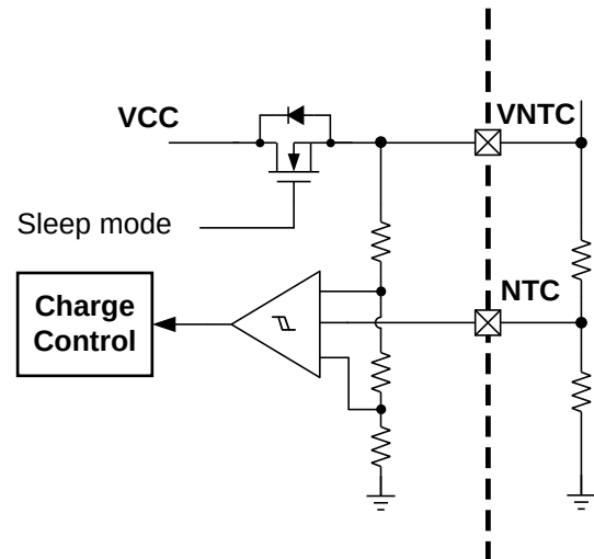
Figure 10: NTC Protection Block
