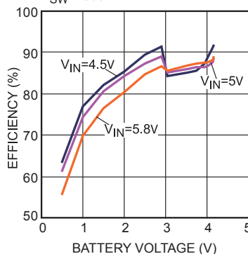
Constant Current Charge Efficiency
