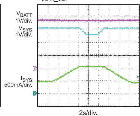
SYS Output Current Limit, Boost Mode
