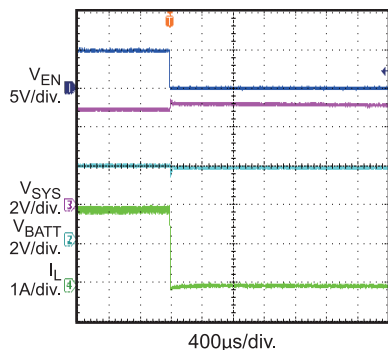
System Short Protection
