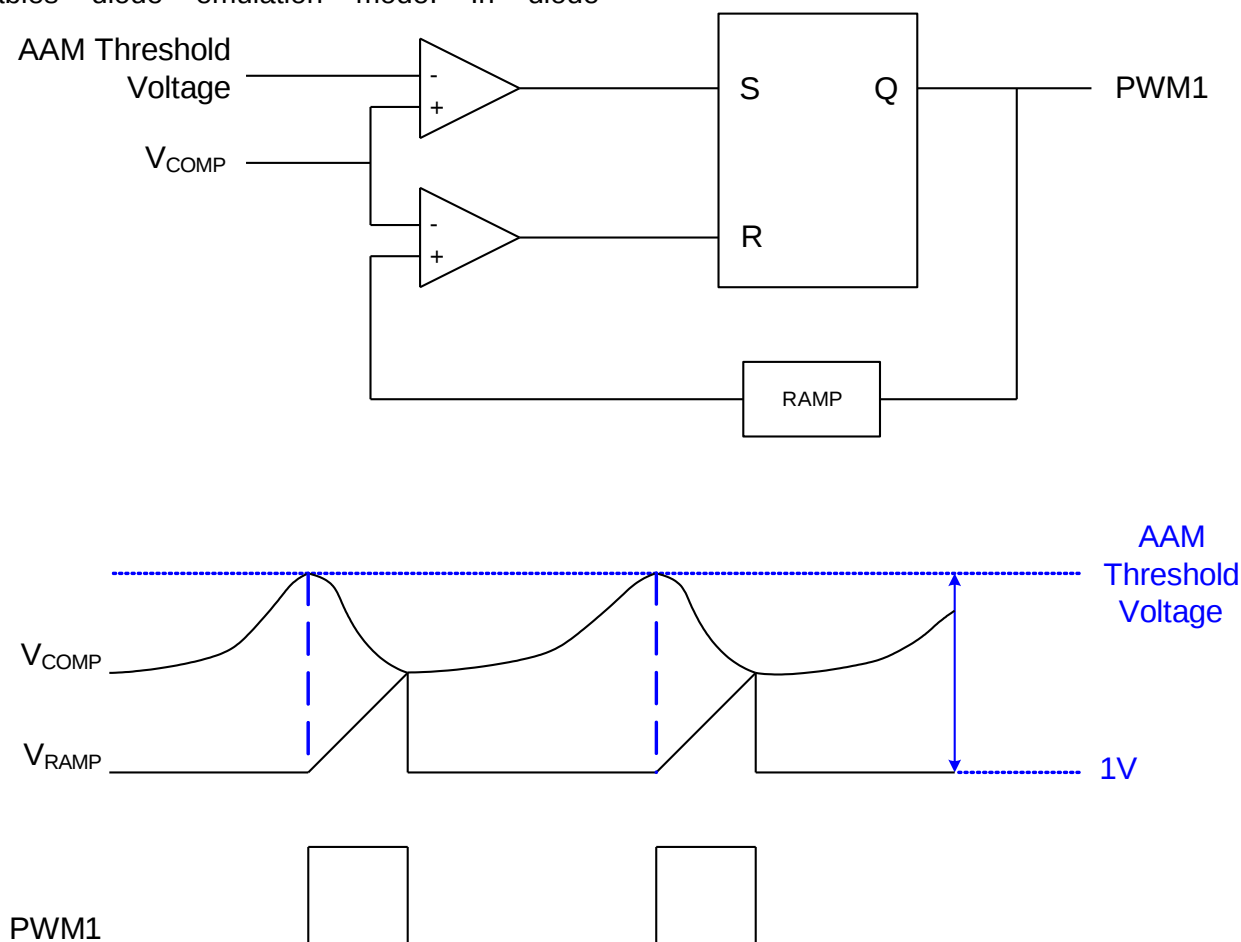
Figure 2: Block Diagram of AAM Operation and Typical Waveforms
