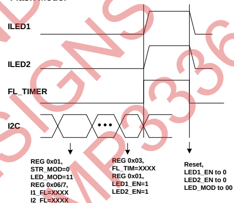
Figure 9: Software and Edge Trigger Flash Mode Torch Mode to Flash Mode
