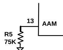
Figure 6—AAM network
