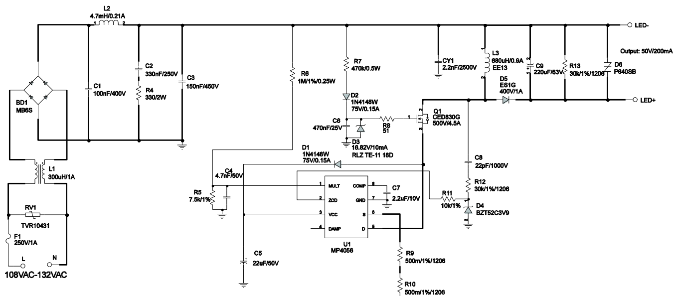
Figure 20: GU10 Bulb Driver, 120VAC/60Hz Input, V_O = 50V , I_O = 200mA , Buck-Boost Converter, Low Bom Cost, EVB Model: EV4056-S-00A
