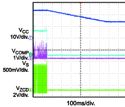
OVP LED Load Open then Recovery V IN =230V AC /50Hz, Full Load
