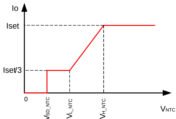
Figure 19: NTC Curve
