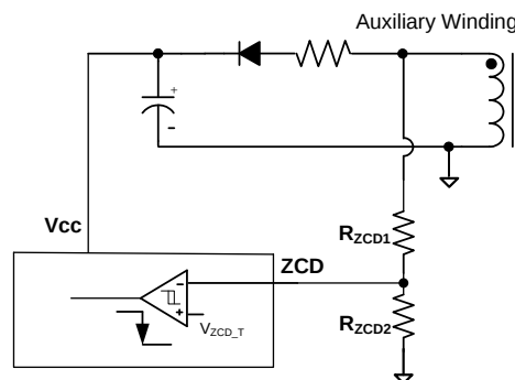
Figure 3: Zero-Current Detector
