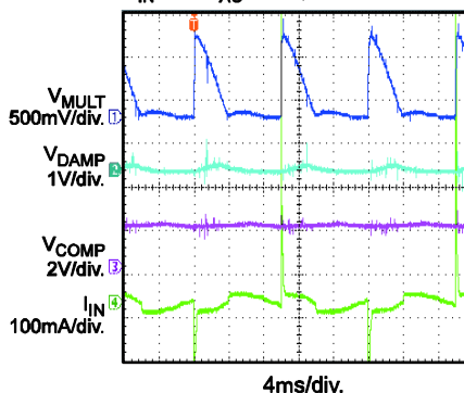
Dimming Performance Min dimming on phase with leading-edge dimmer V IN =230V AC /50Hz, with dimmer
