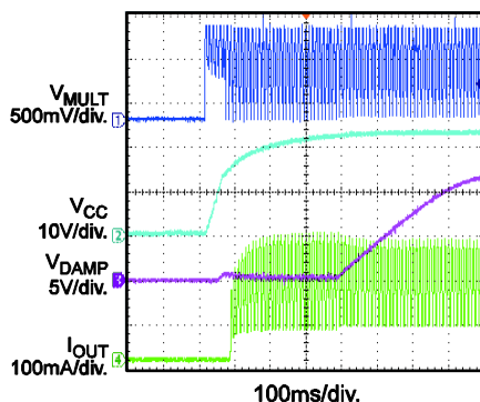
V IN Start Up V IN =230V AC /50Hz, Full Load
