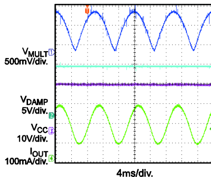
Steady State V IN =230V AC /50Hz, Full Load
