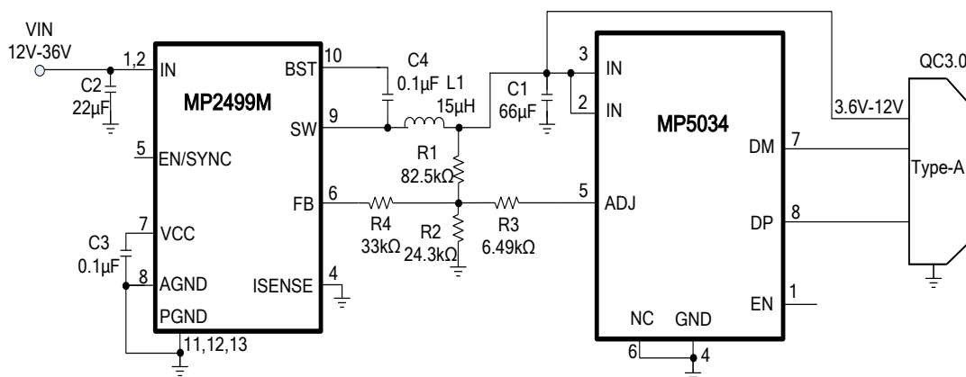
Figure 7: MP5034 + MP2499M for CLA Car Charger
