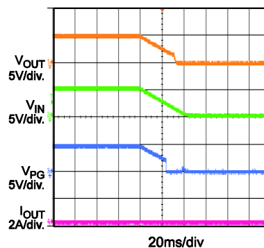
VIN Shutdown (Load Switch)
