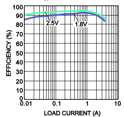
Efficiency CH1, V_{IN}=3.3V
