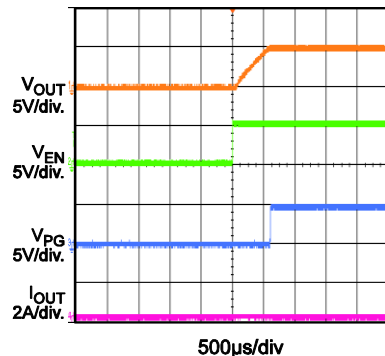
EN Start-Up (Load Switch)
