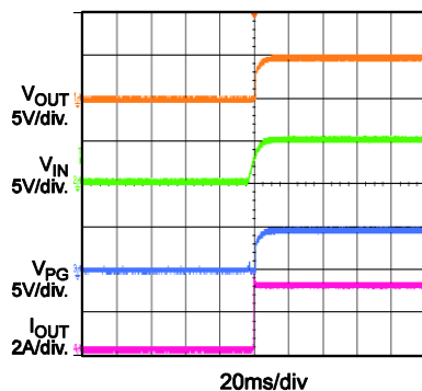
VIN Start-Up (Load Switch)
