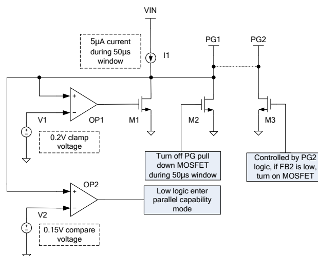
Figure 3: PG Functional Schematic
