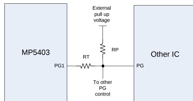
Figure 4: PG Connection Example
