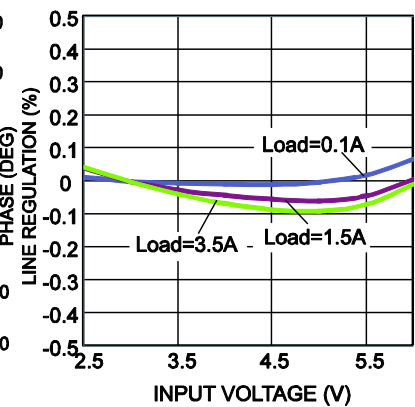
Line Regulation CH1
