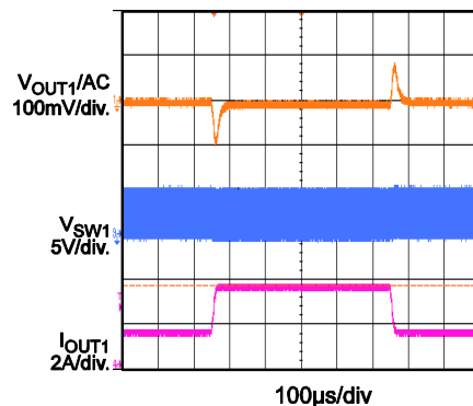
CH1 Transient
