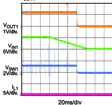
VIN Power Down without
