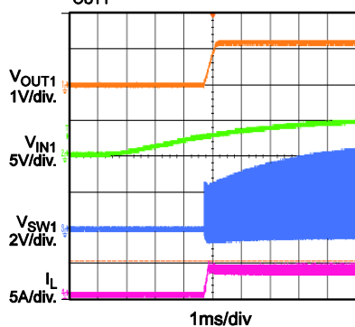
VIN Power Up with 3.5A
