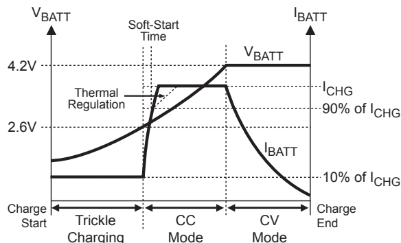
Figure 2—Charger Typical Charging Procedure
