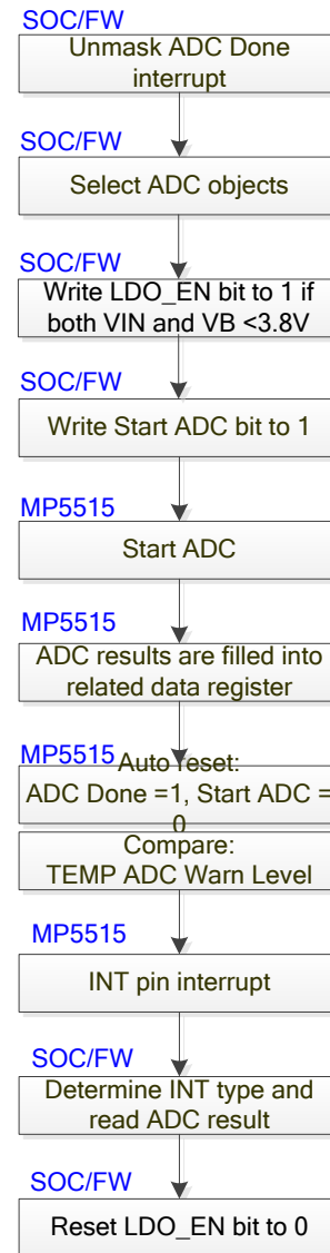
Figure 7: ADC Converter Work Flow
