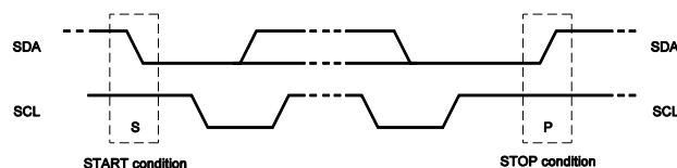
Figure 10: Start and Stop Conditions
