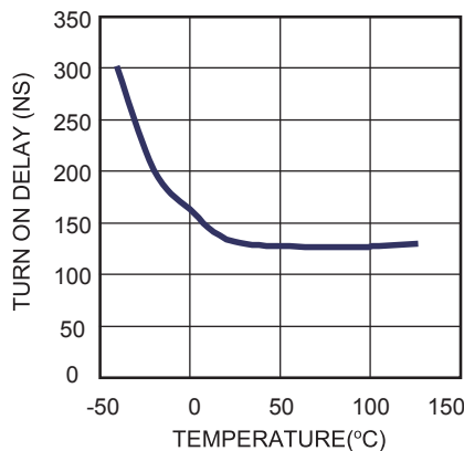
Turn On Delay (Load=10nF) vs. Temperature
