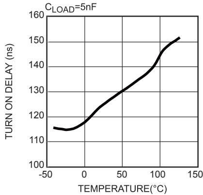
Turn-On Delay vs. Temperature
