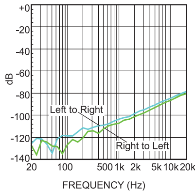
Cross Talk (16V, 8Ω+66μH, P_{OUT}=5W )
