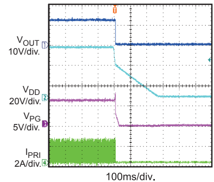
VDD Shutdown
