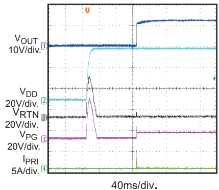
VDD Start-Up
