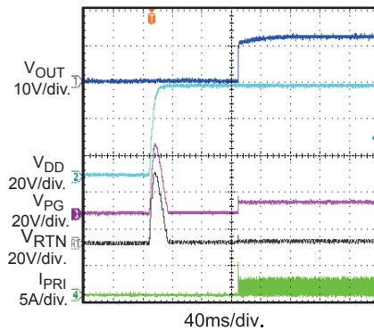
VDD Start-Up
