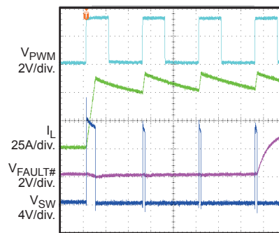
HS Current Limit
