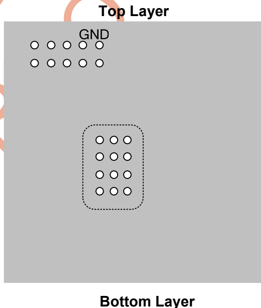
Figure 4—PCB Layout
