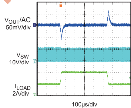
Load Transient Response I_{OUT}=2A to 4A
