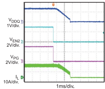
Shutdown through EN2
