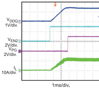
Start-Up through EN2
