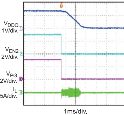
Shutdown through EN2
