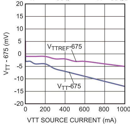
VTT Source Current Load Regulation
