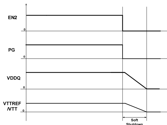
Figure 8: Soft Shutdown Sequence
