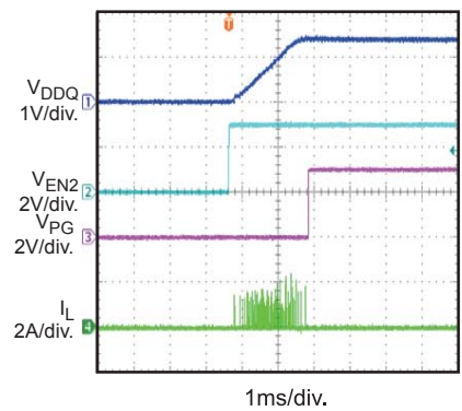
Start-Up through EN2
