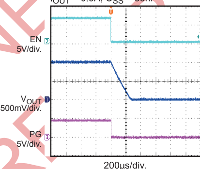
Power Good through EN Shutown
