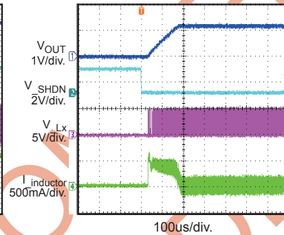
SHDN Start up without Load
