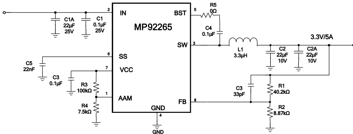
Figure 8: 12 V_{IN} , 3.3V/5A
