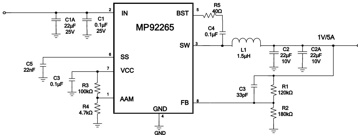
Figure 9: 12 V_{IN} , 1V/5A (9)
