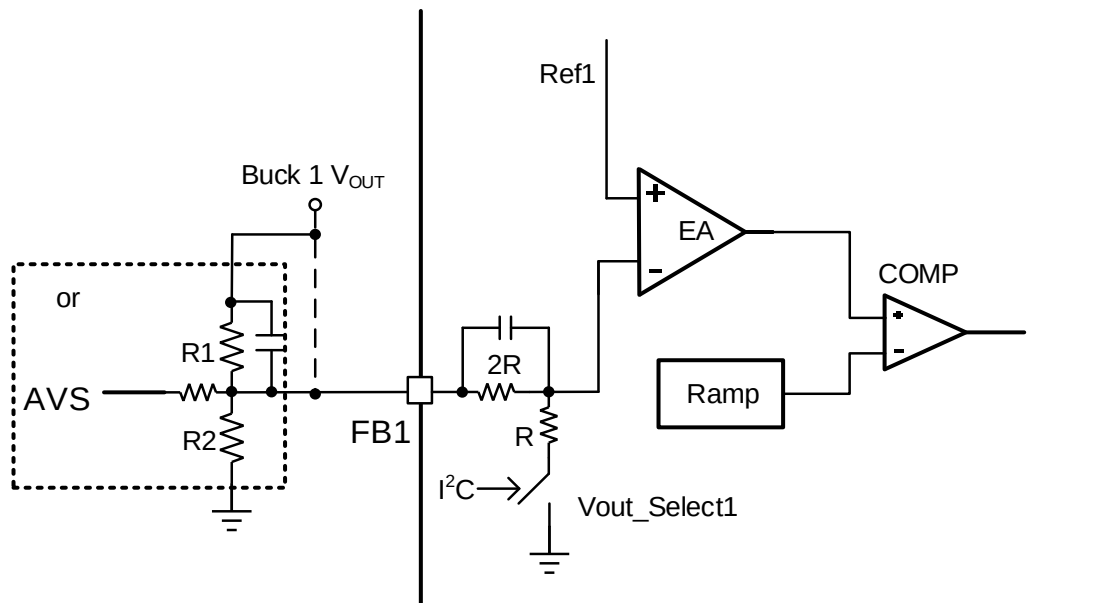
Figure 5: Output Voltage Setting
