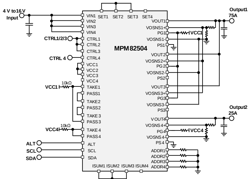
Figure 11: Typical Application Circuit (4V to 16V Input, 75A Output in Parallel Operation plus 25A Output)
