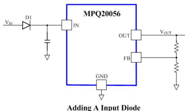
Adding A Input Diode
