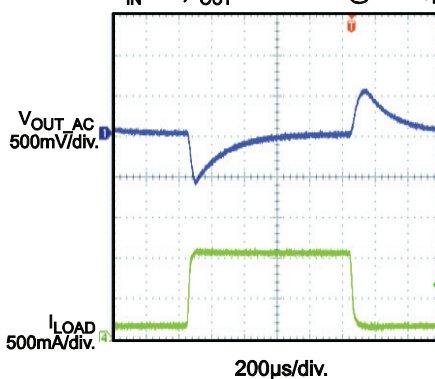
Response to Transient Load
