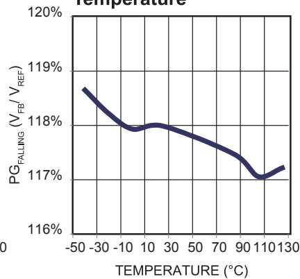
PG Falling Thershold ( V_{FB} Rising) vs. Temperature
