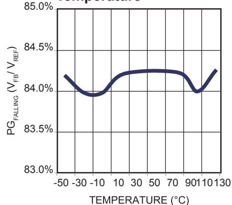
PG Falling Threshold (V FB Falling) vs. Temperature
