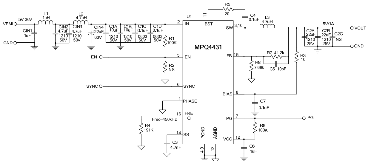
Figure 17: Application Circuit with EMI Filter @ V_{OUT} = 5V/1A , F_{SW} = 450kHz
