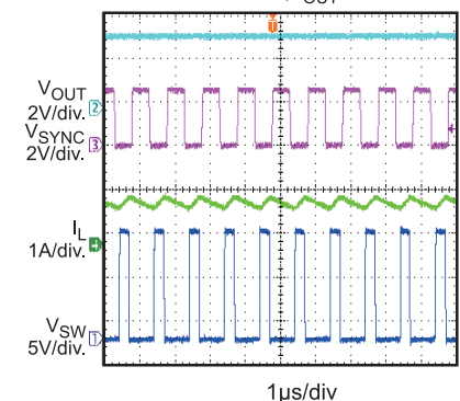
SYNC Operation (180° Out-of-Phase)
