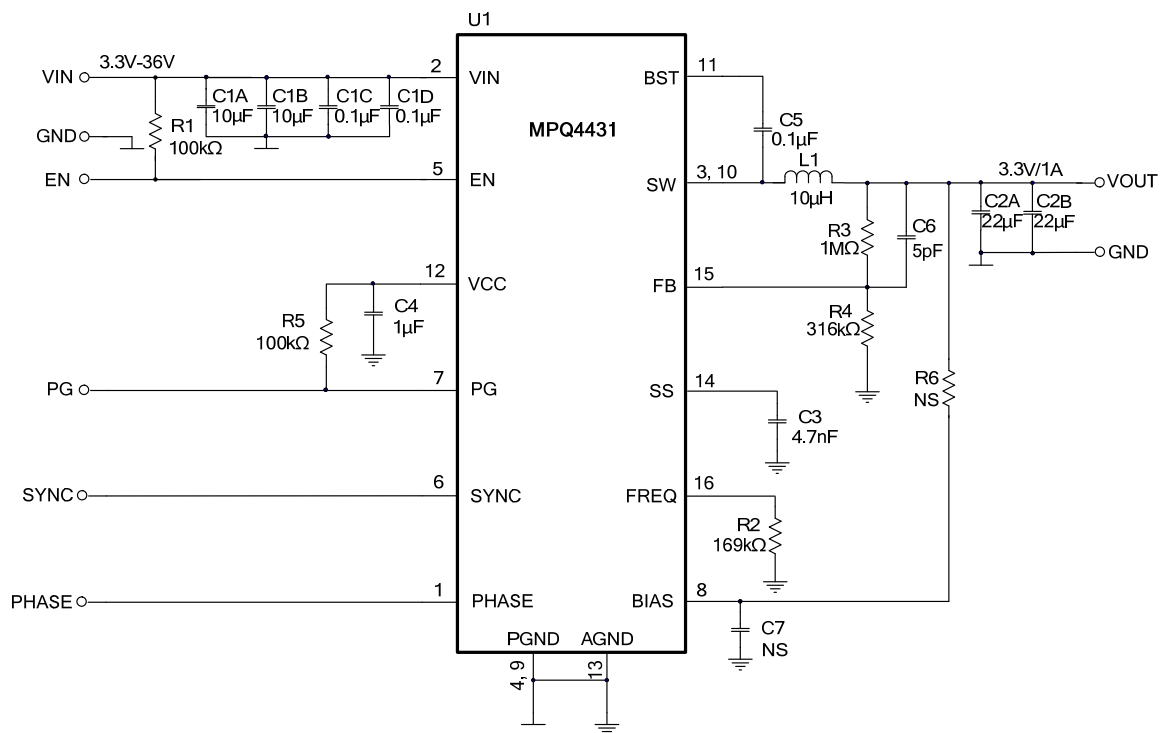
Figure 9: V_{OUT} = 3.3V , I_{OUT} = 1A , F_{sw} = 500kHz
