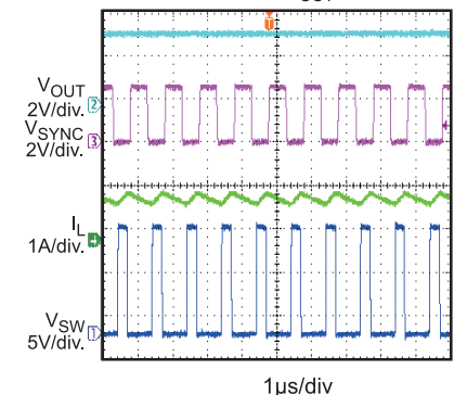
SYNC Operation (180° Out-of-Phase)
