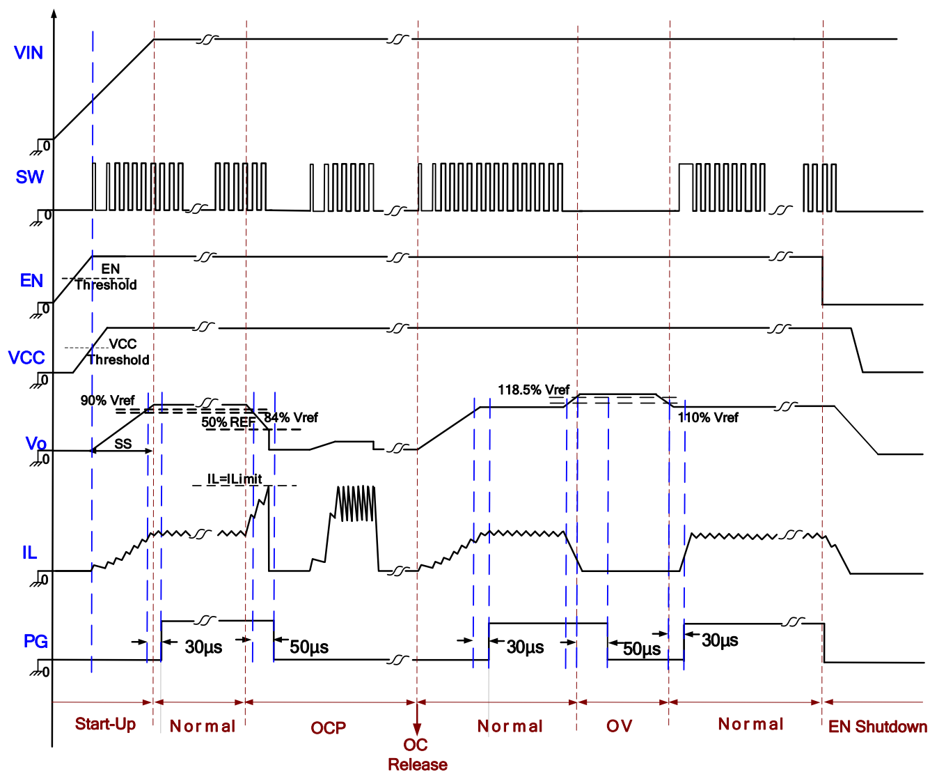
Figure 2: Timing Sequence
