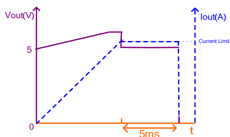
Figure 7: Over-Current Limit
