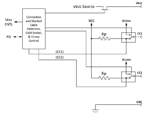
Figure 10: CC Functional Block
