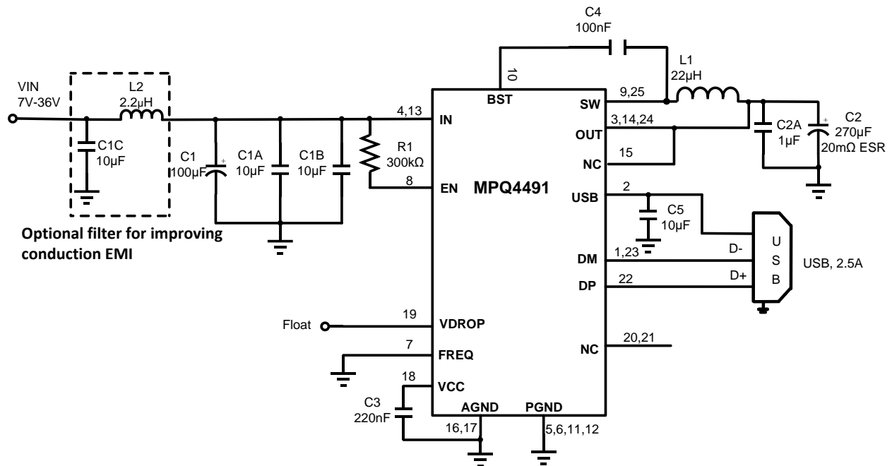
Figure 6: V_{IN} = 7V - 36V , USB = 5V/2.5A
