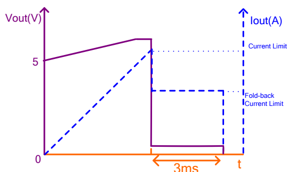
Figure 4: Over-Current Limit
