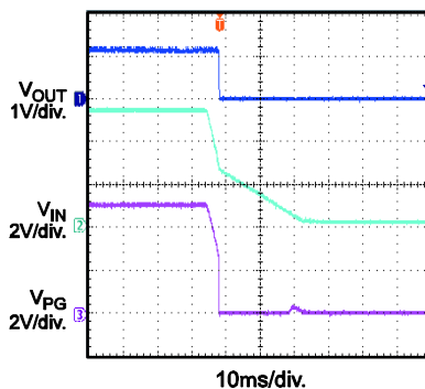
Power Good Through Vin Shutdown I_{OUT}=12A
