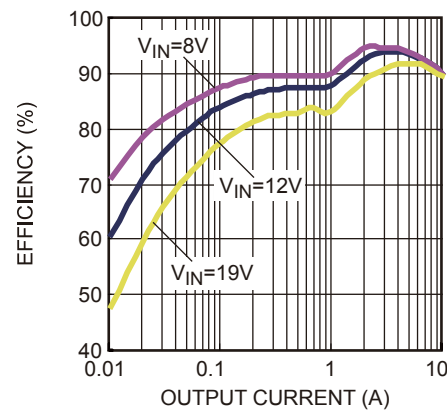
Figure 32 — Efficiency Curve
