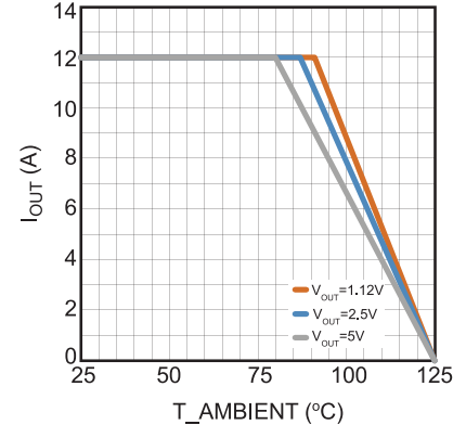
Thermal Derating
