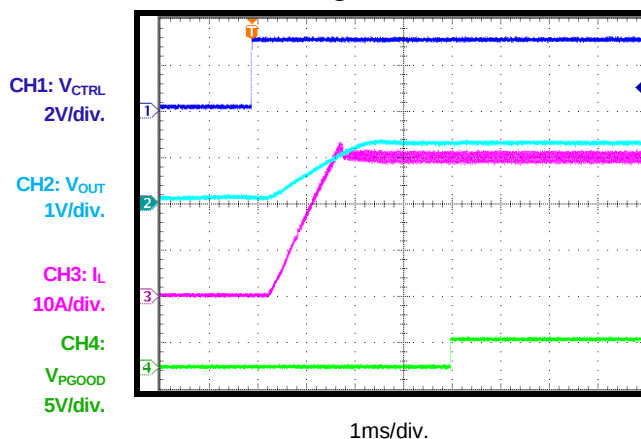
Power-On through CTRL, DCM, I_{OUT} = 30A , Single-Phase
