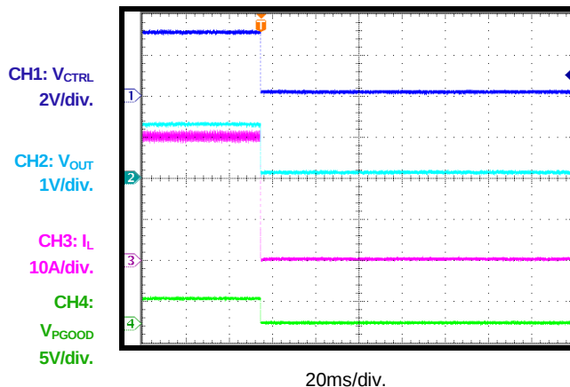
Power-Off through CTRL, DCM, I_{OUT} = 30A , Single-Phase
