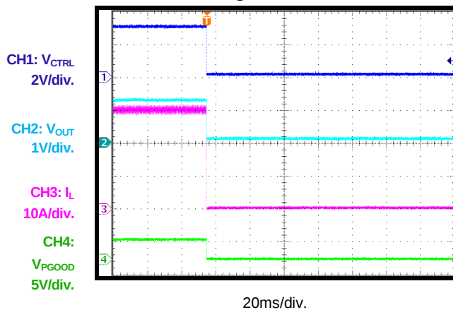
Power-Off through CTRL, CCM, I_{OUT} = 30A , Single-Phase
