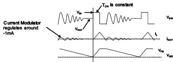
Figure 3: Light-Load Operation
