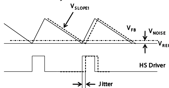
Figure 5: Jitter in PWM Mode
