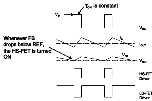
Figure 2: Heavy-Load Operation
