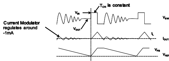
Figure 3: Light-Load Operation
