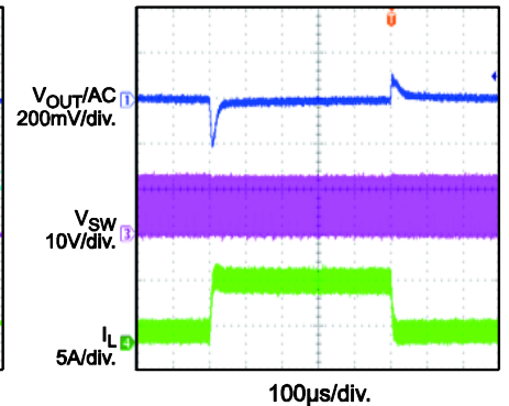
Transient V_{IN} = 12V , L = 1.5\mu H , C_{OUT} = 88\mu F I_{OUT} = 1.2A-6.8A @ 1.6A/\mu s
