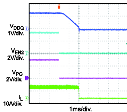
Shutdown Through EN2
