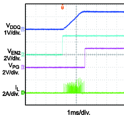
Start-Up through EN2
