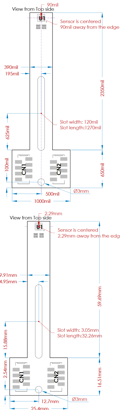
Figure 9: LT Type 1 Mechanical Drawing, mil = 0.001" = 0.0254mm
