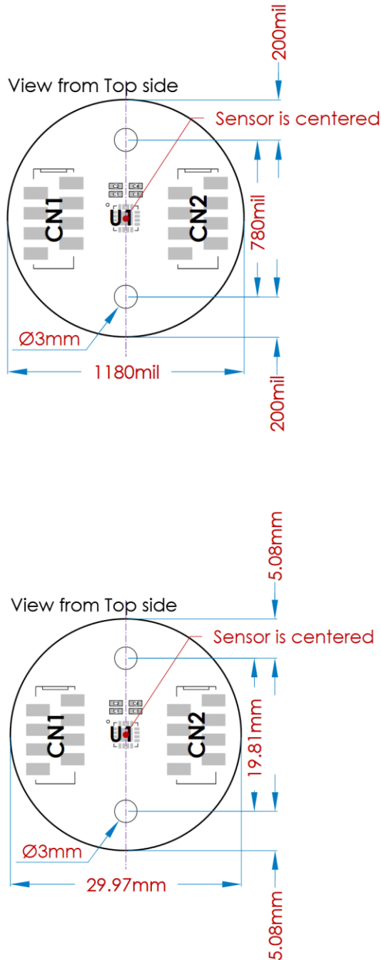
Figure 8: RD Type 1 Mechanical Drawing Not Recommended for New Designs, Refer to LT Type 1 Mechanical Drawing
